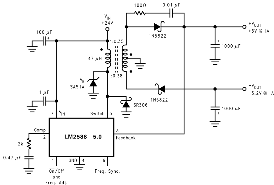
Figure 58. Flyback Regulator
